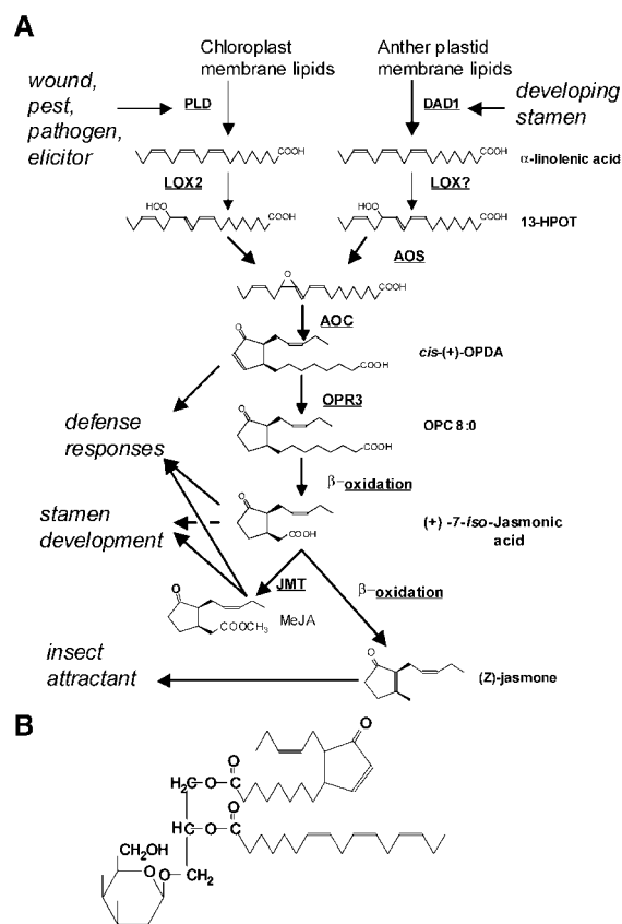
Figure 2. Model for the Biosynthesis of JAs.
