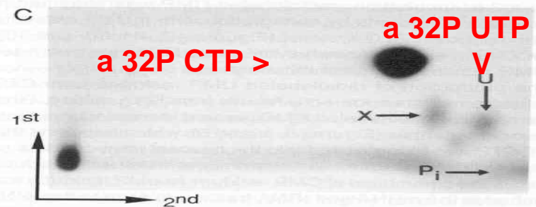
Figure 5. Two-Dimensional Fractionation of NMPs from Petunia Mitochondrial Transcripts.
