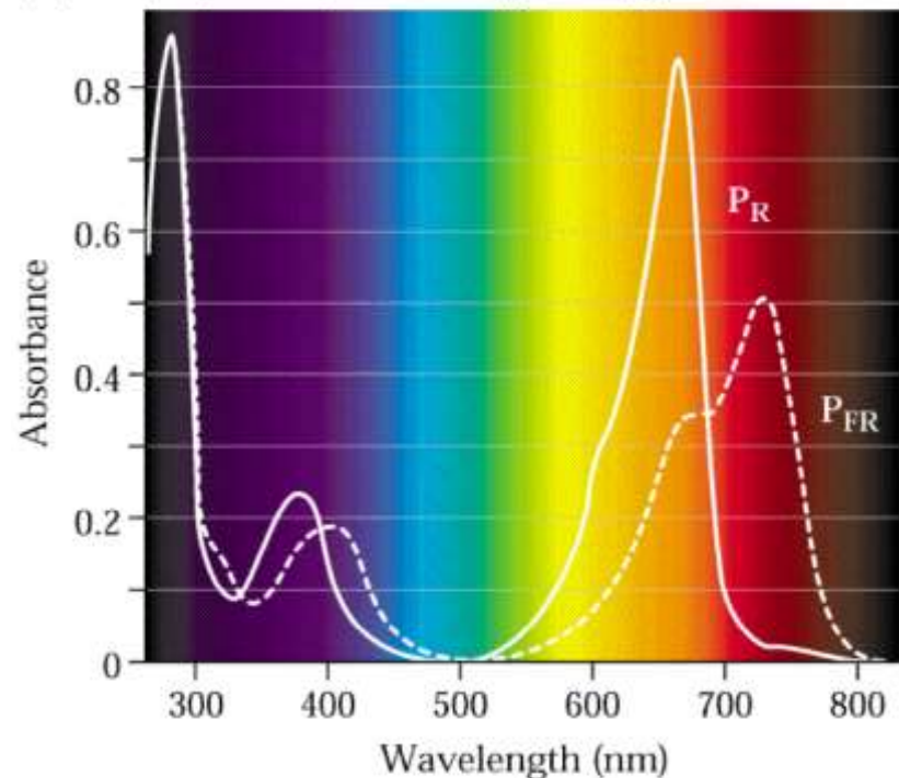
(C) Absorption spectra of P_R and P_{FR}
