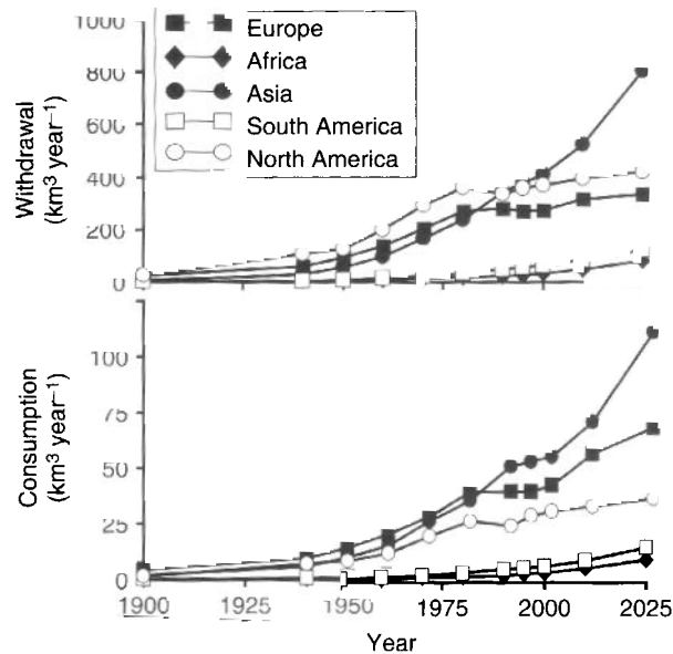
Figure 8 Withdrawal and consumption of water for industrial and domestic purposes as a function of time for various continents. Data after 1995 is projected (Data taken from Shiklomanov, 1997).
